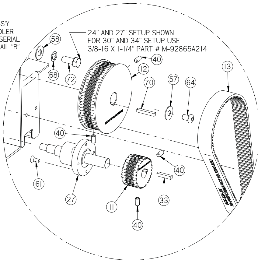
DETAIL A
