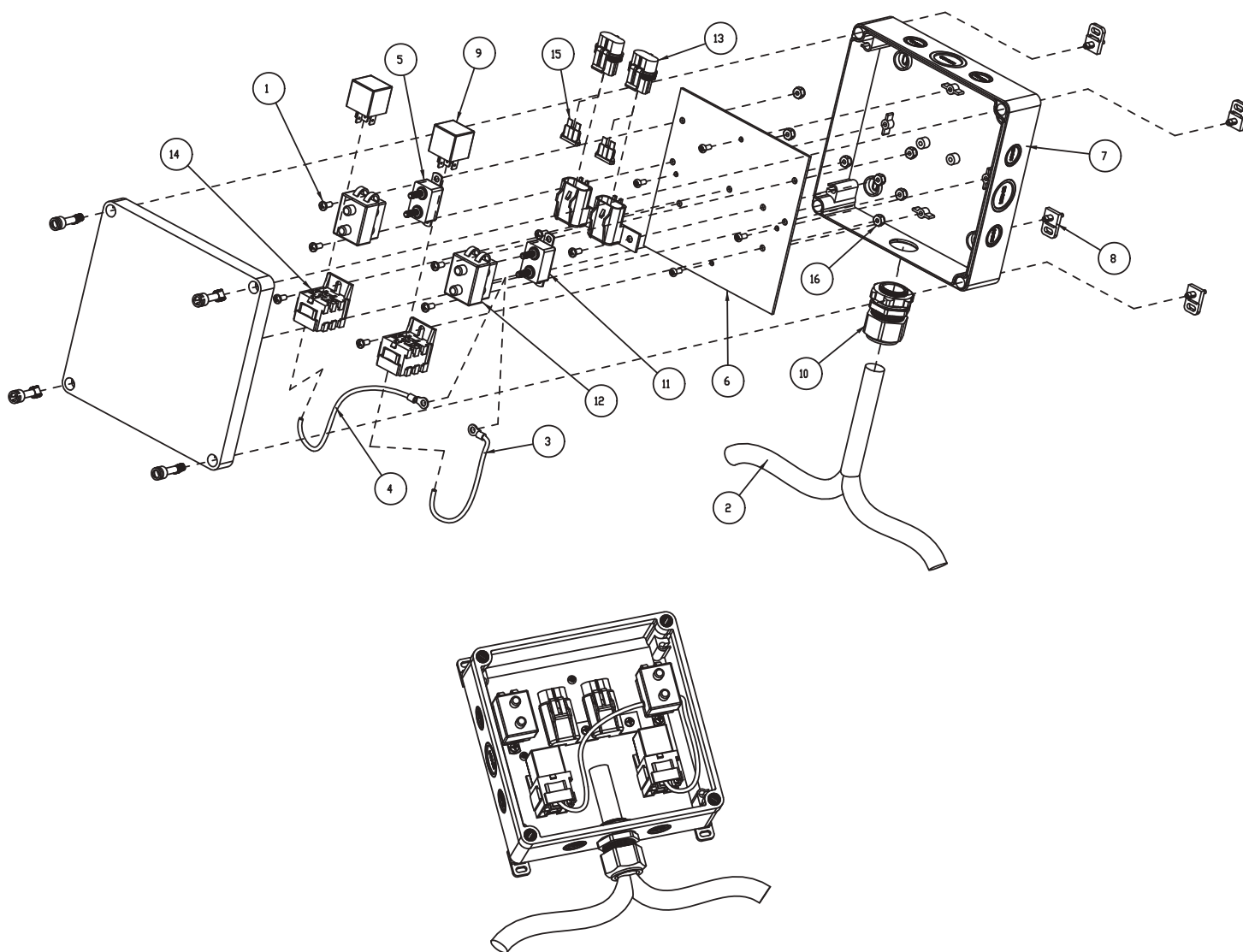
CONTROL BOX SHOWN WITHOUT TOP COVER
